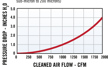
FIGURE 3 - Pressure drop of 1.1 inches of water at 1,000 CFM air flow.
